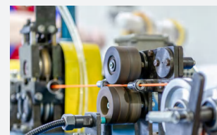
Wire stripping machine
