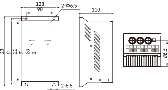
Dimensions of BR100-045 braking unit
