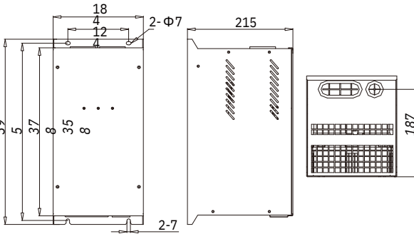
Dimensions of BR100-315\BR100-400 braking unit
