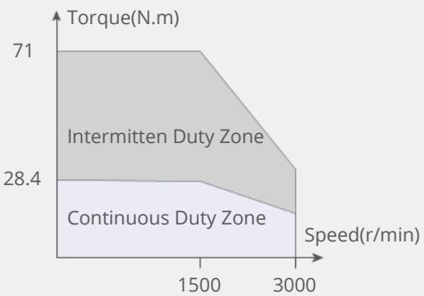
4400W Motor
