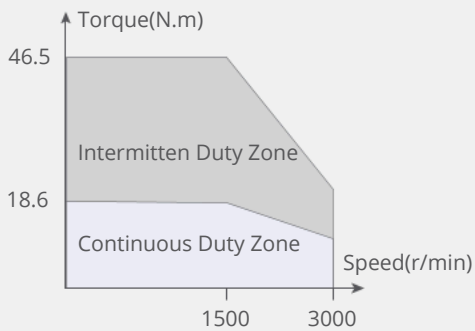
2900W Motor
