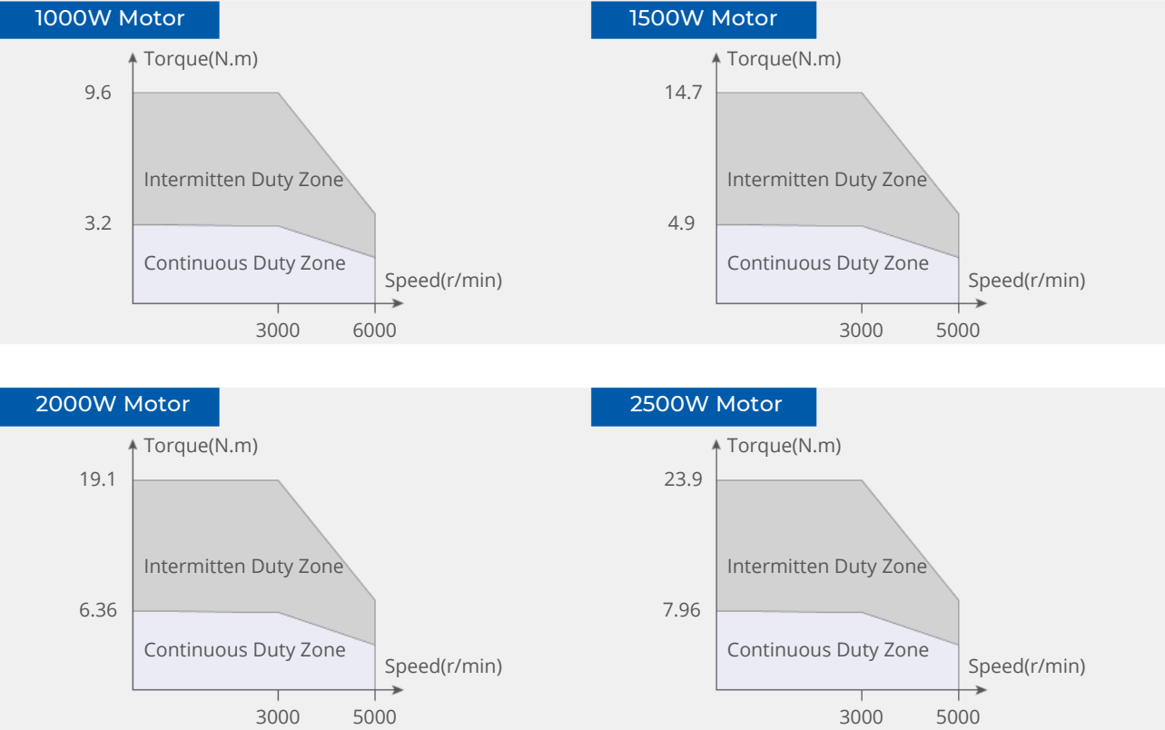
Speed-Torque characteristics
