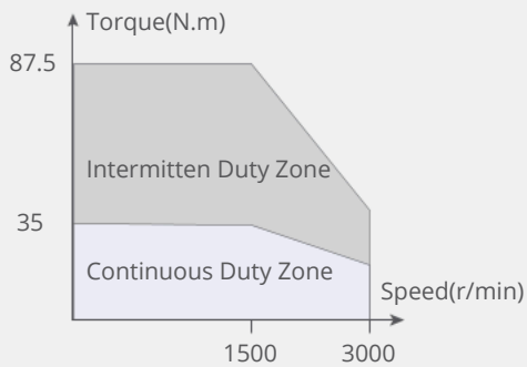
5500W Motor
