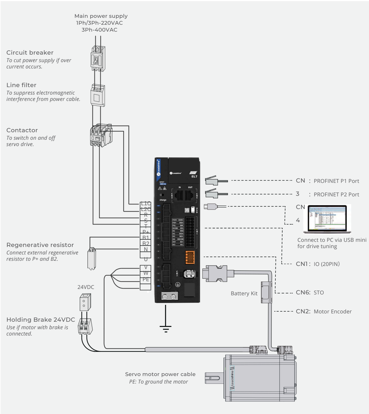
EL7-PN & Peripheral Wiring Diagram
