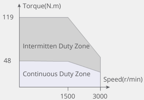
7500W Motor
