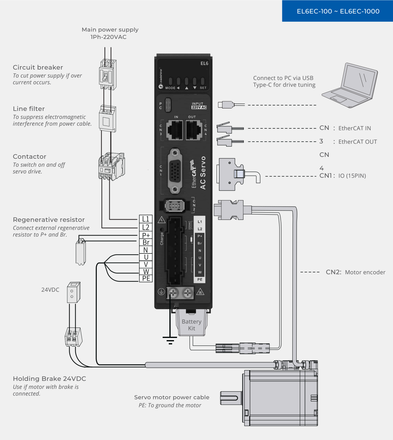
EL6-EC & Peripheral Wiring Diagram
